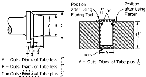
FIG. A2.11 Flaring Tool and Die Block for Flange Test Note 1—Metric equivalent: 1 in. = 25.4 mm.
