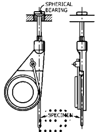
FIG. A4.2 Snubbing-Type Gripping Device
