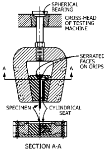
FIG. A4.1 Wedge-Type Gripping Device
