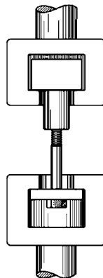
FIG. A3.1 Tension Testing Full-Size Bolt
