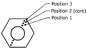
FIG. A3.7 Hardness Test Locations
