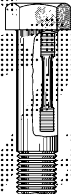
FIG. A3.5 Location of Standard Round 2-in. Gauge Length Tension Test Specimen When Turned from Large Size Bolt
