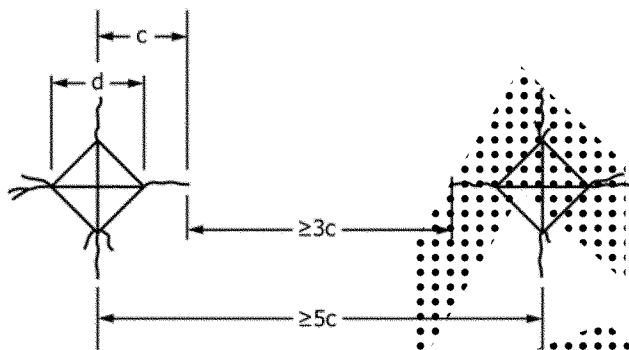
FIG. 3 Closest Permitted Spacing for Vickers Indentations
