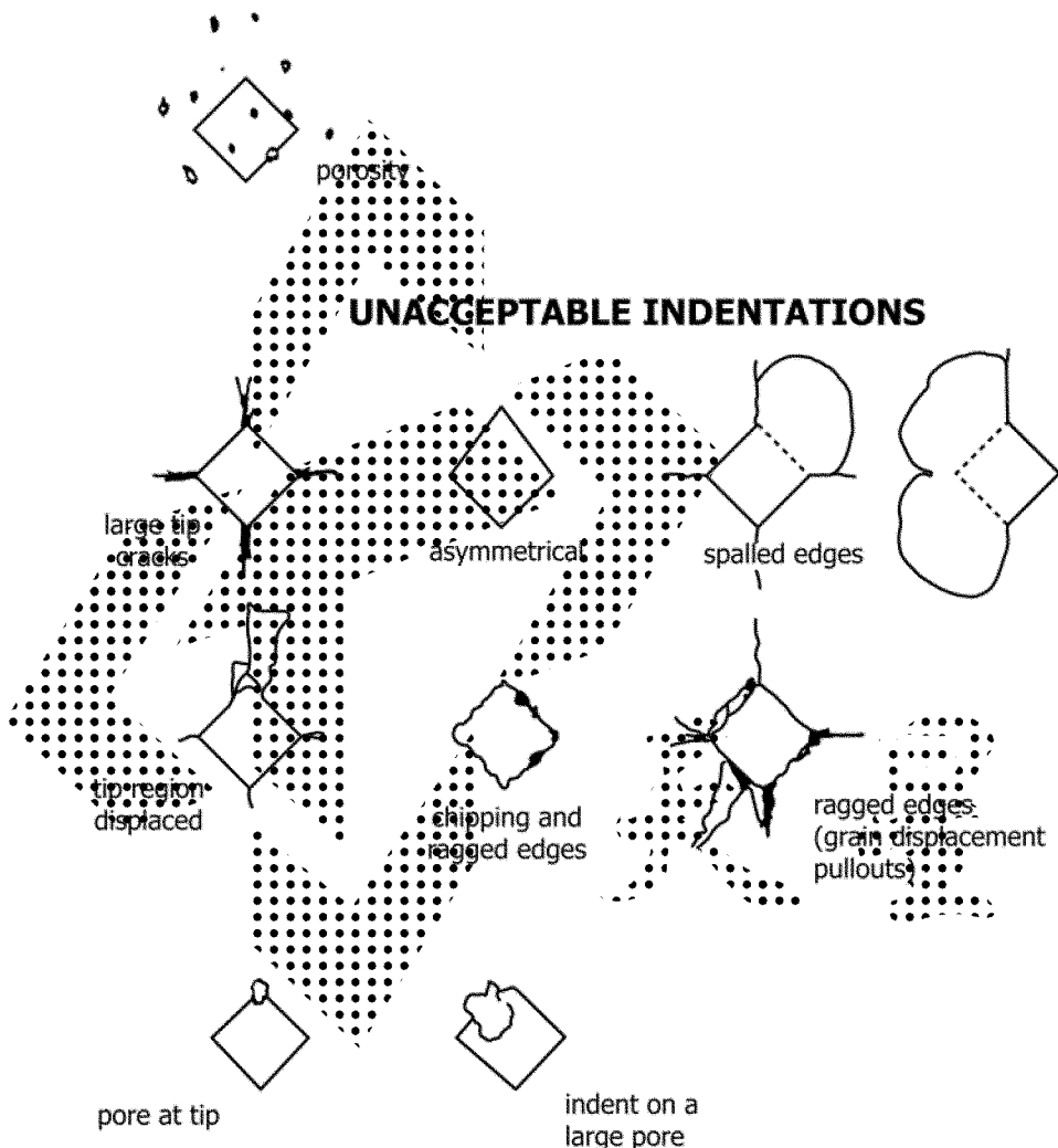
FIG. 4 Guidelines for the Acceptance of Indentations
